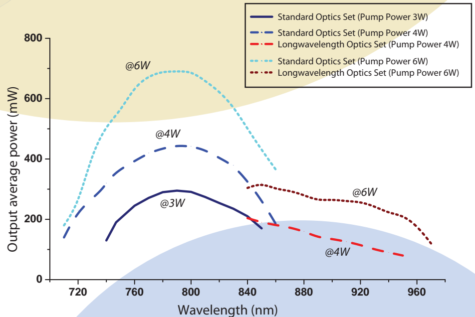
Trestles wavelength tuning curves
