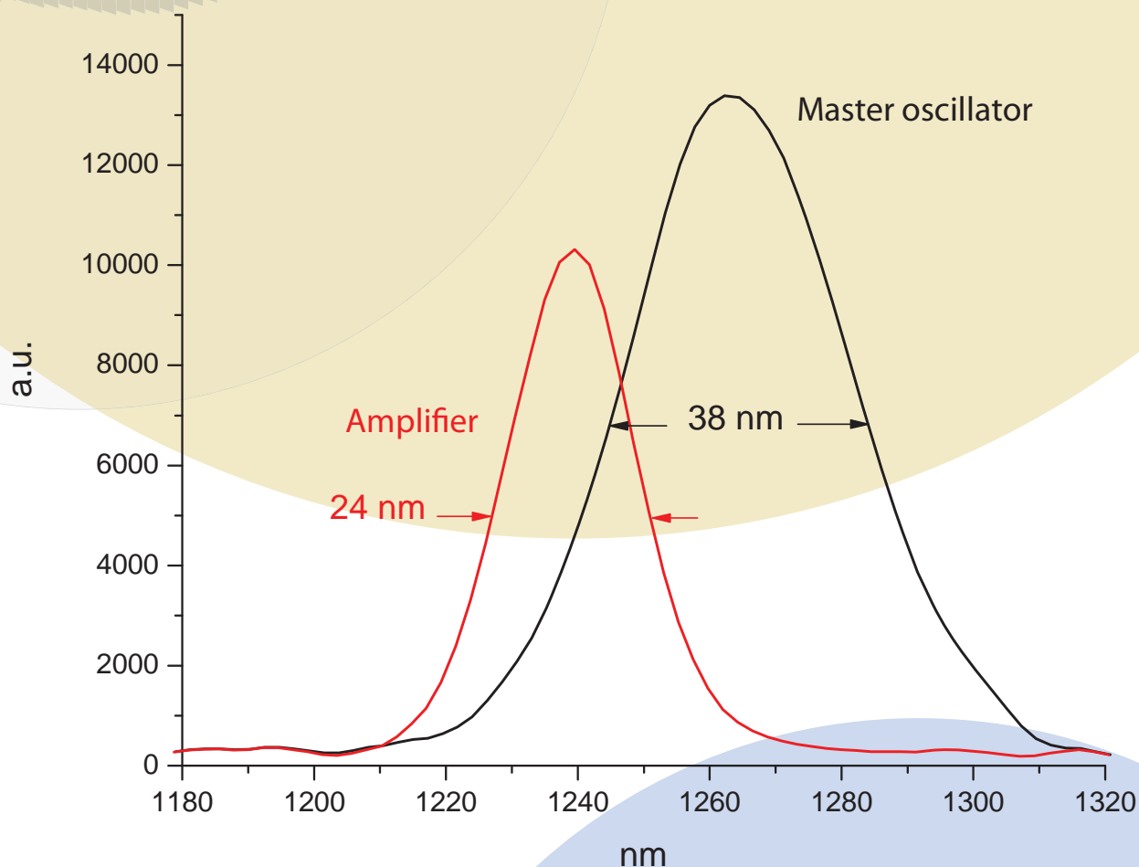
Spectra of the Cortes-200 system
