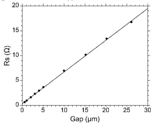
Figure 6. TLM results of regrown processed contacts with 25 μm width, regrown on 100 μm thick InGaAs:Si with n=3.6 \times 10^{19} \text{ cm}^{-3} .
