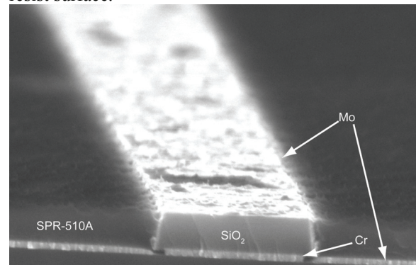
Figure 3. SEM of SPR 510-A sample after thinning in an ICP.
