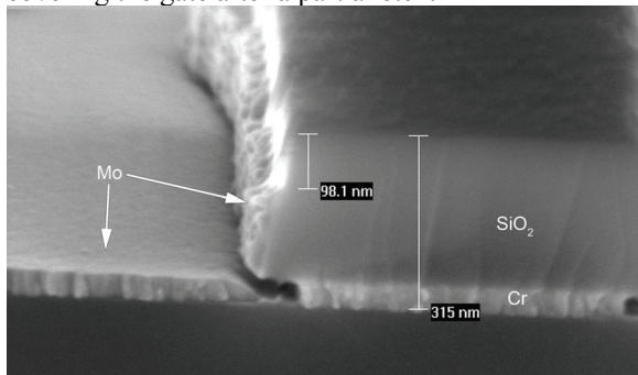
Figure 5. SEM close up of Mo sidewall remaining on gate after resist was stripped
