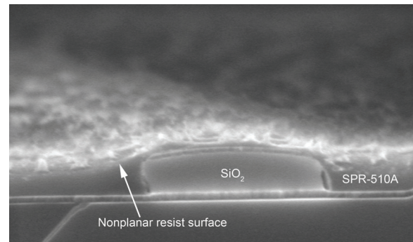
Figure 2. SEM of SPR 510-A sample after thinning in a capacitively coupled plasma, producing a nonplanar resist surface.
