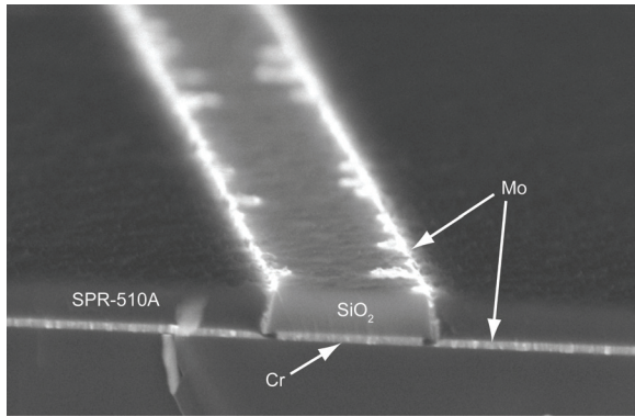
Figure 4. SEM shows Molybdenum as the bright area covering the gate after a partial etch.
